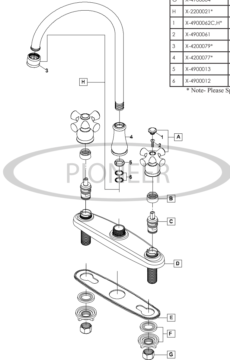
Product Diagram
